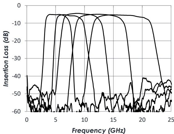
Typical Frequency Response
