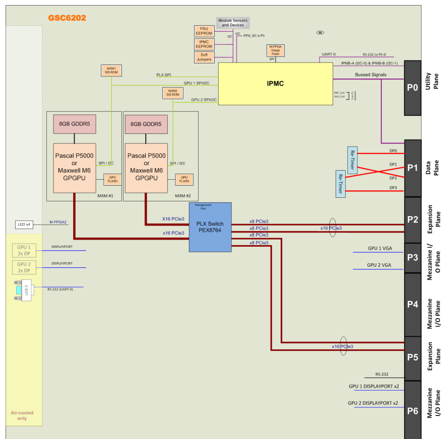
Figure 1. GSC6202 functional block diagram
