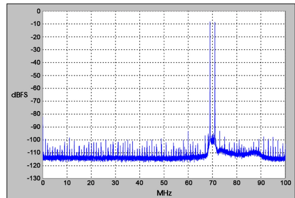
Two-Tone SFDR
