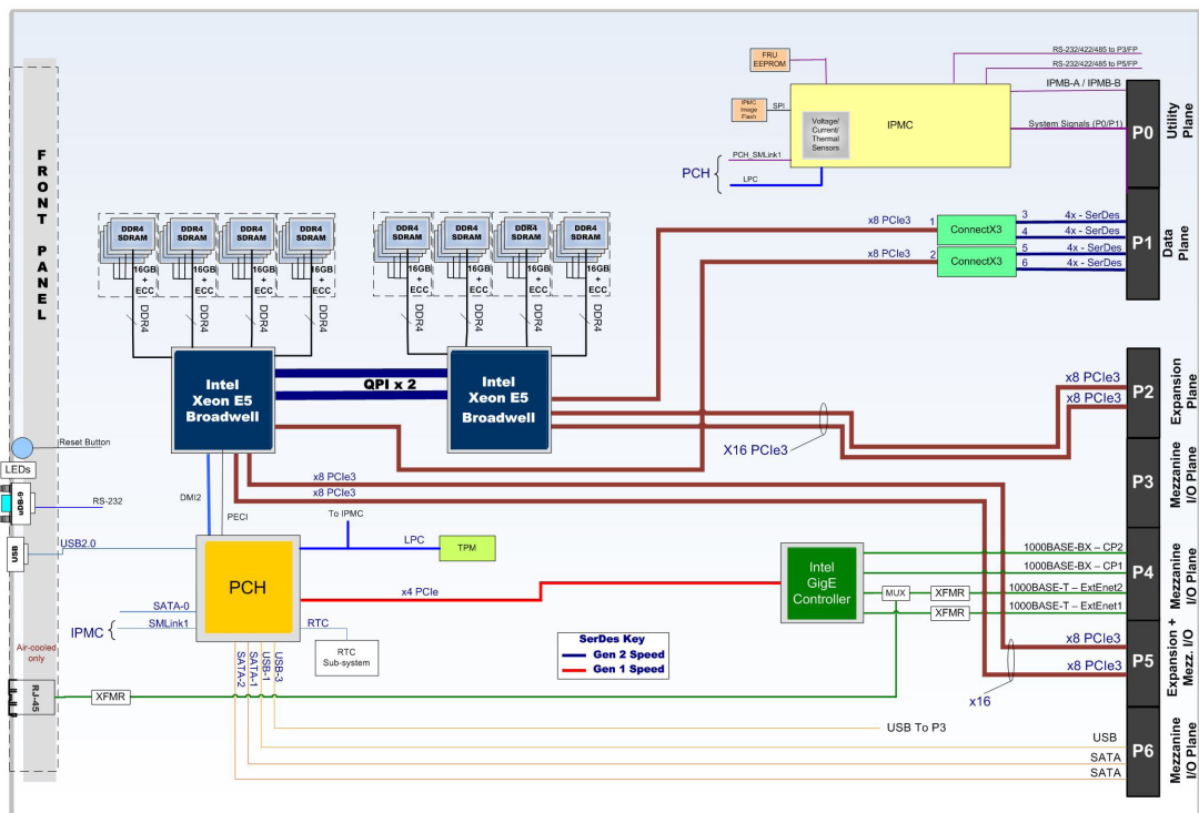
HDS6603B functional block diagram
