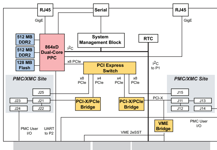
Figure 1. VME SBC4120 Module functional block diagram
