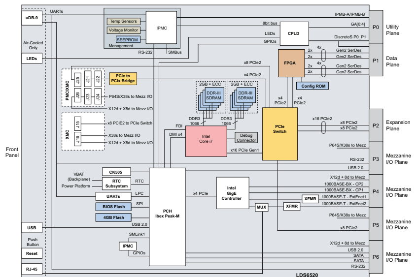
Figure 1. LDS6520 Module functional block diagram
