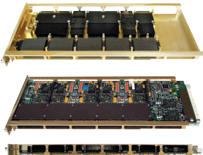
Example of ManagedAir board cover and mounted board
