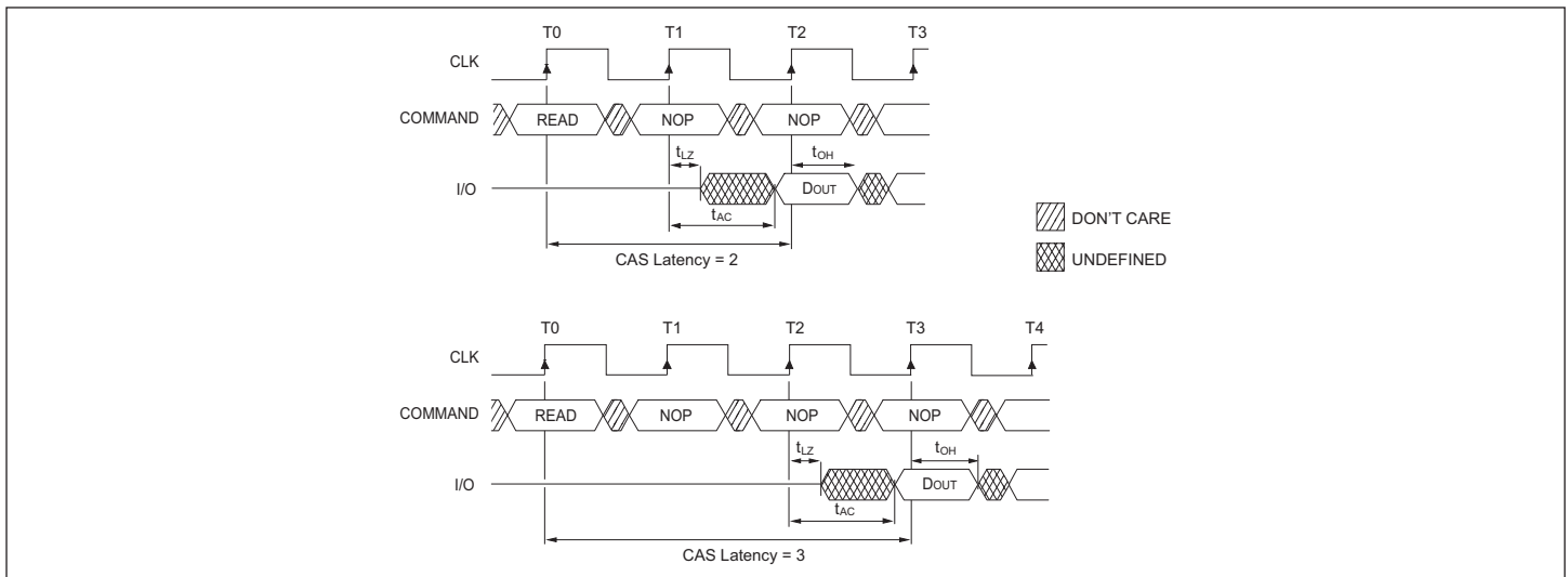
FIGURE 4 – CAS LATENCY
