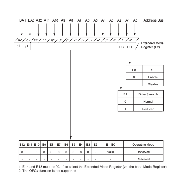
FIGURE 5 – EXTENDED MODE REGISTER DEFINITION
