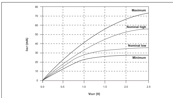
FIGURE C – REDUCED DRIVE PULL-DOWN CHARACTERISTICS
