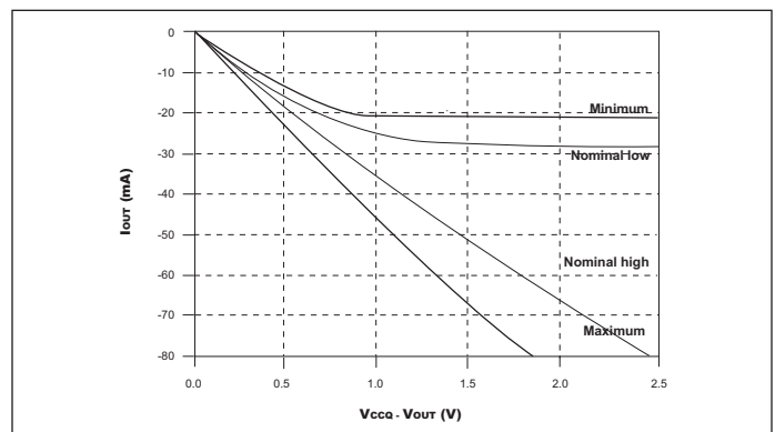
FIGURE D – REDUCED DRIVE PULL-UP CHARACTERISTICS
