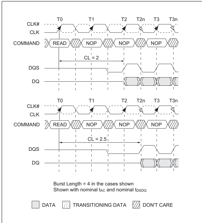
FIGURE 4 – CAS LATENCY
