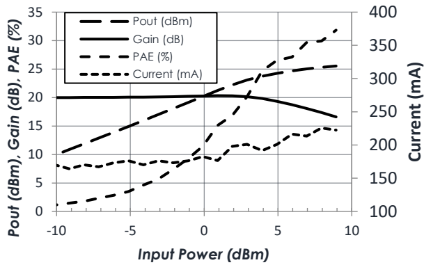
Power Compression at 12 GHz
