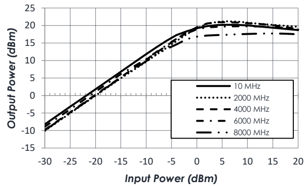
Pin vs. Pout, VDD = +5V
