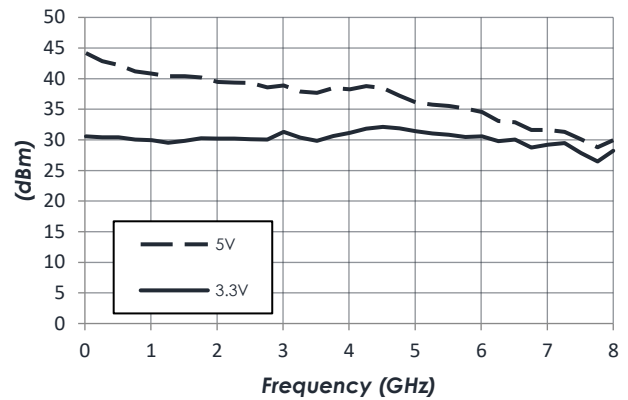
Output IP2 vs VDD
