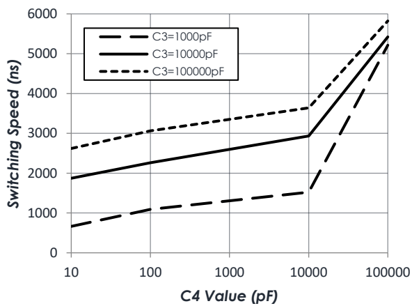
Bypass to Amp On vs Cap Values
