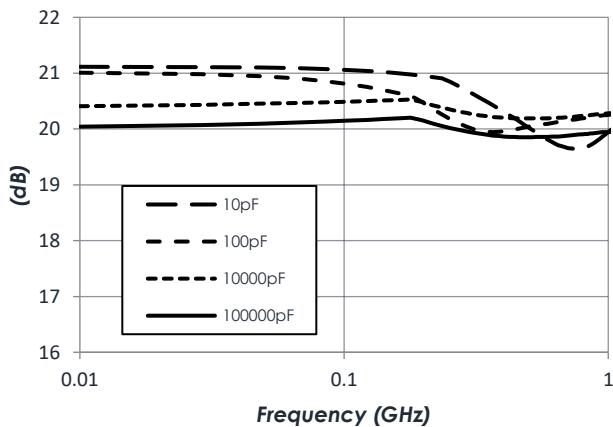
Gain vs C4 Value
