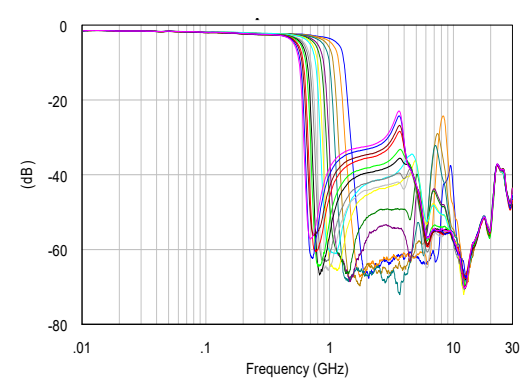
DC Couple Low Pass Mode
