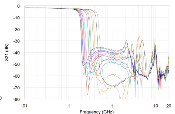
DC-Coupled Low Pass Mode
