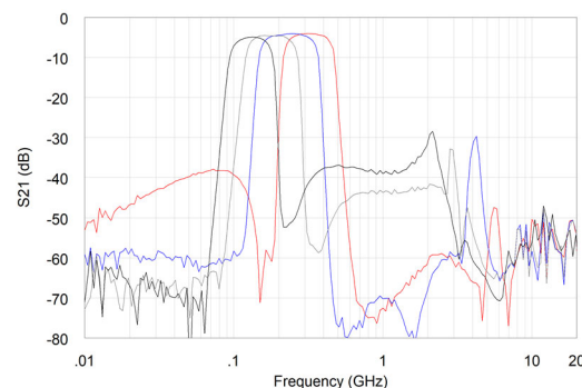
Adjustable Center Frequency
