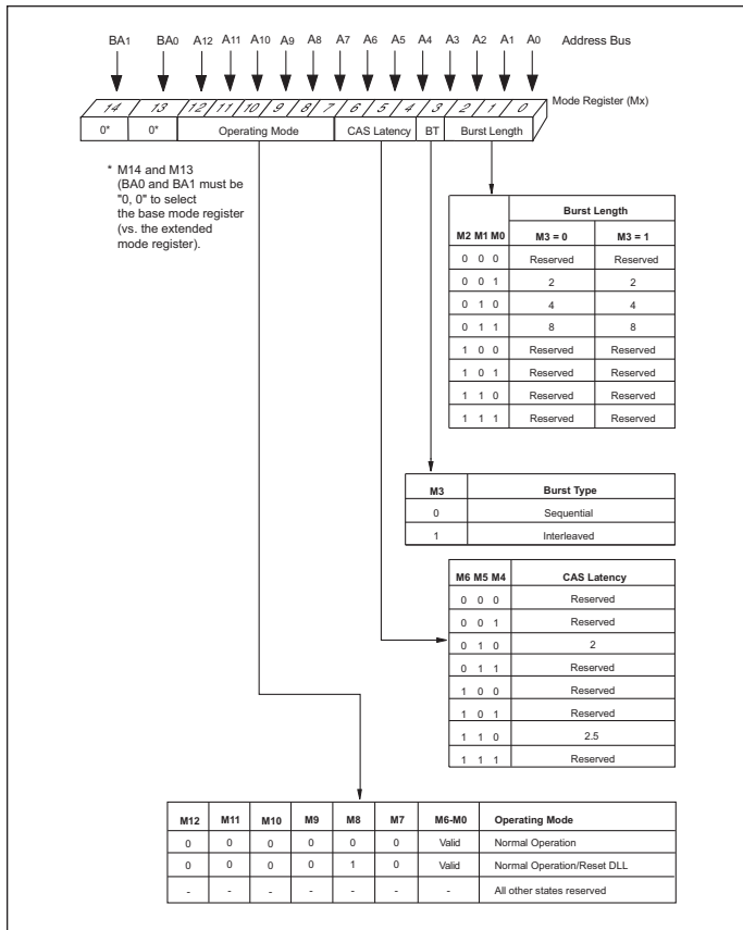
FIGURE 3 – MODE REGISTER DEFINITION
