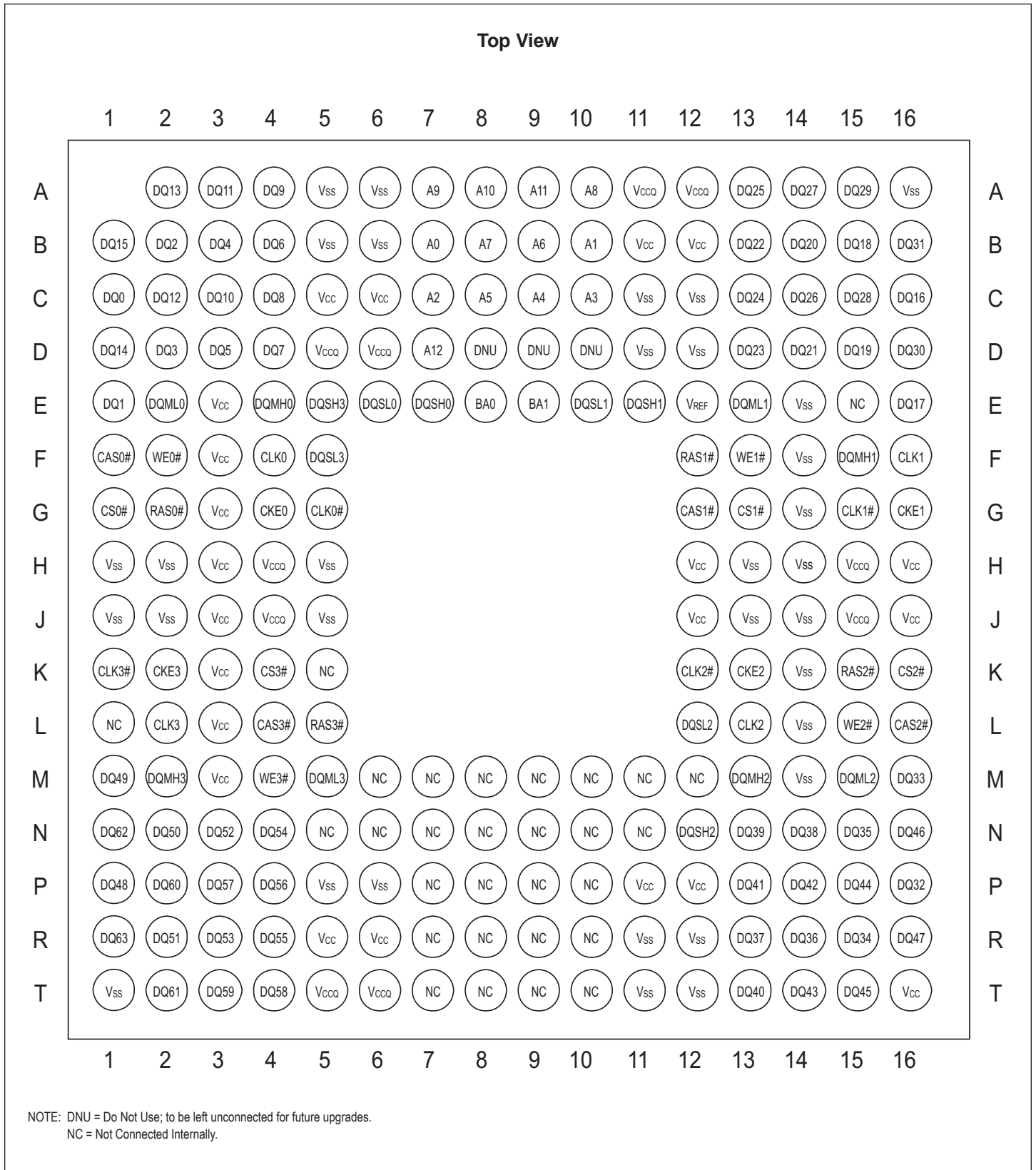
FIGURE 1 – PIN CONFIGURATION
