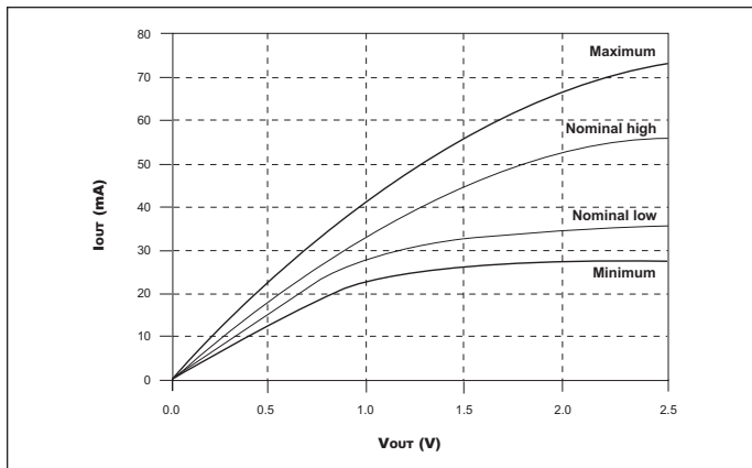
FIGURE C – PULL-DOWN CHARACTERISTICS
