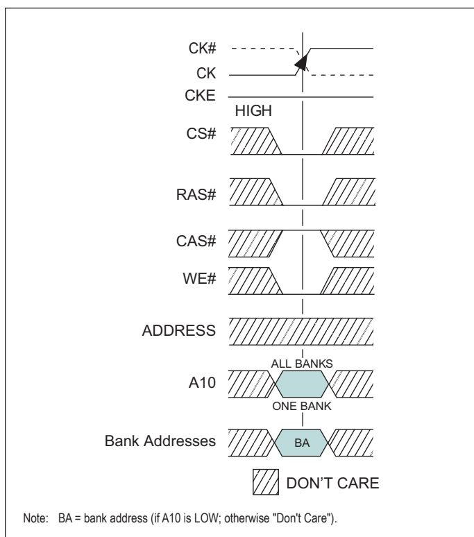
FIGURE 13 – PRECHARGE COMMAND
