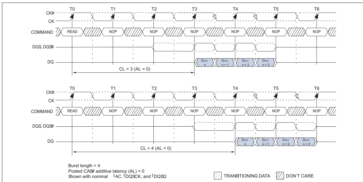
FIGURE 6 – CAS LATENCY (CL)
