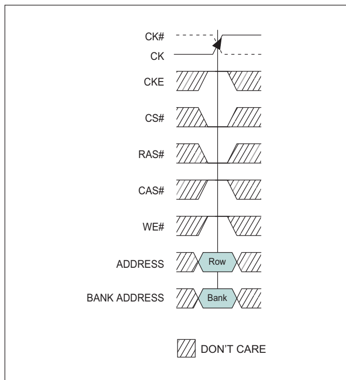
FIGURE 10 – ACTIVE COMMAND
