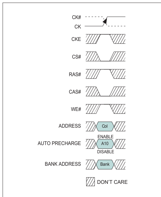
FIGURE 11 – READ COMMAND
