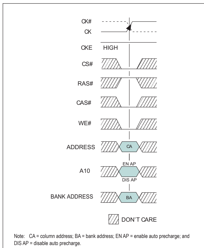
FIGURE 12 – WRITE COMMAND
