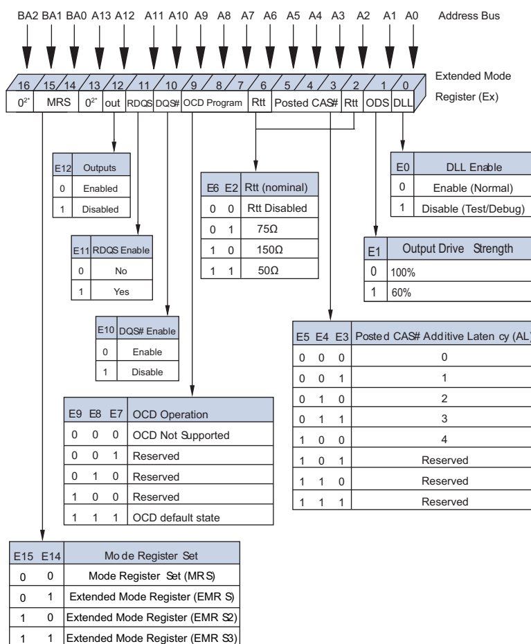
FIGURE 7 – EXTENDED MODE REGISTER DEFINITION
