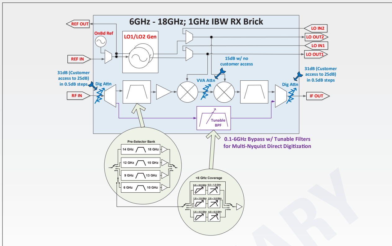
Figure 1. RFM6101 Rx Filtering Block Diagram
