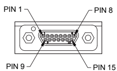
DETAIL A PIN LAYOUT SCALE 5 : 2
